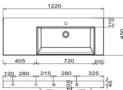
Q!flat 1220 - police vlevo
