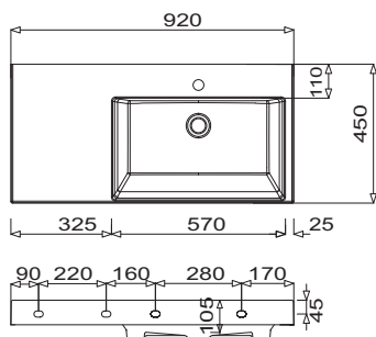
Q!flat 920 - police vlevo
